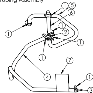
Drain/Fill Tubing Assembly
