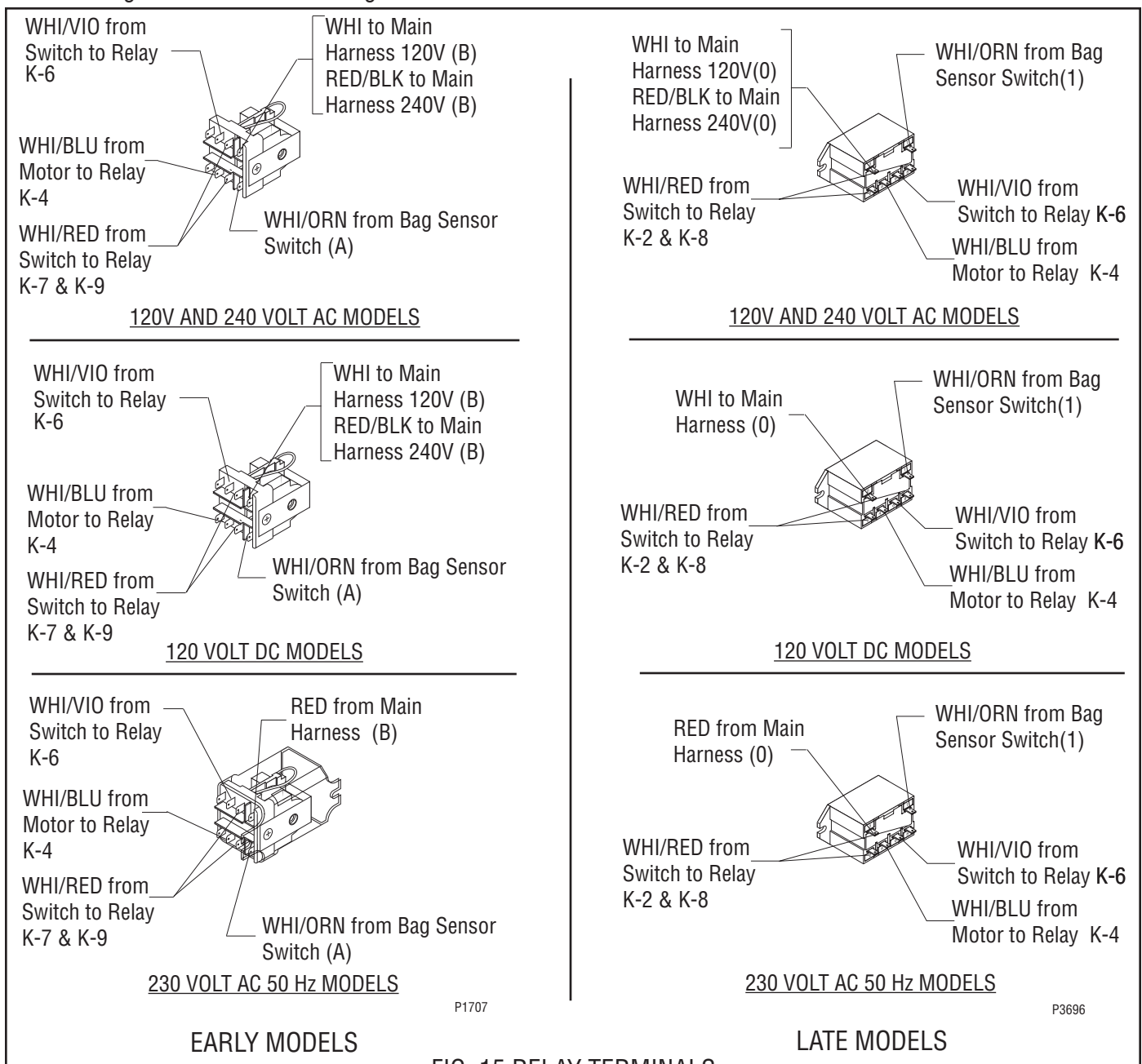
FIG. 15 RELAY TERMINALS
