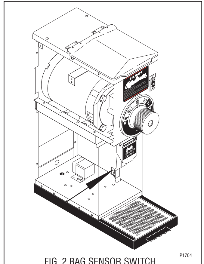
FIG. 2 BAG SENSOR SWITCH
