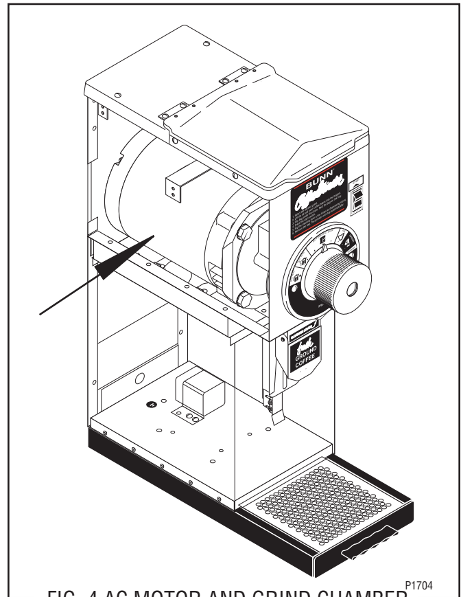
FIG. 4 AC MOTOR AND GRIND CHAMBER
