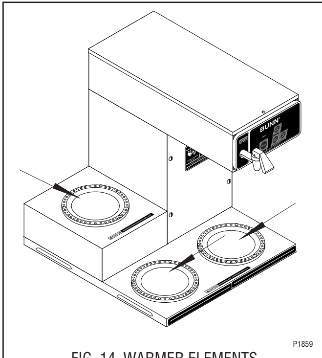
FIG. 14 WARMER ELEMENTS
