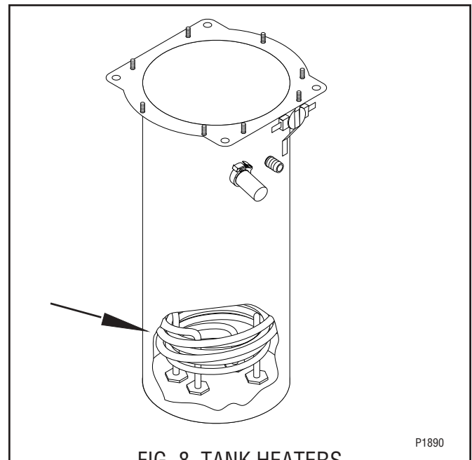
FIG. 8 TANK HEATERS
