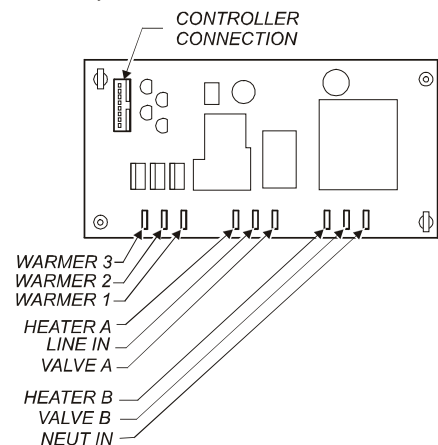
Fig. 21 Power Board Hook-Up
